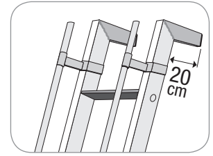
Welded spacers (Code S15/D15)
